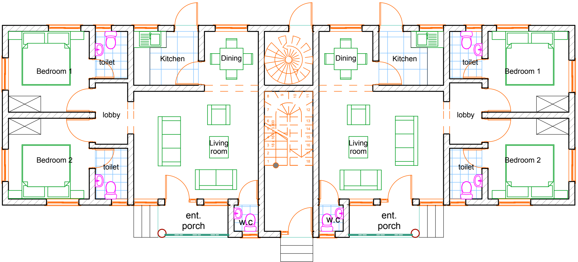
GROUND FLOOR (BLOCK 1)
