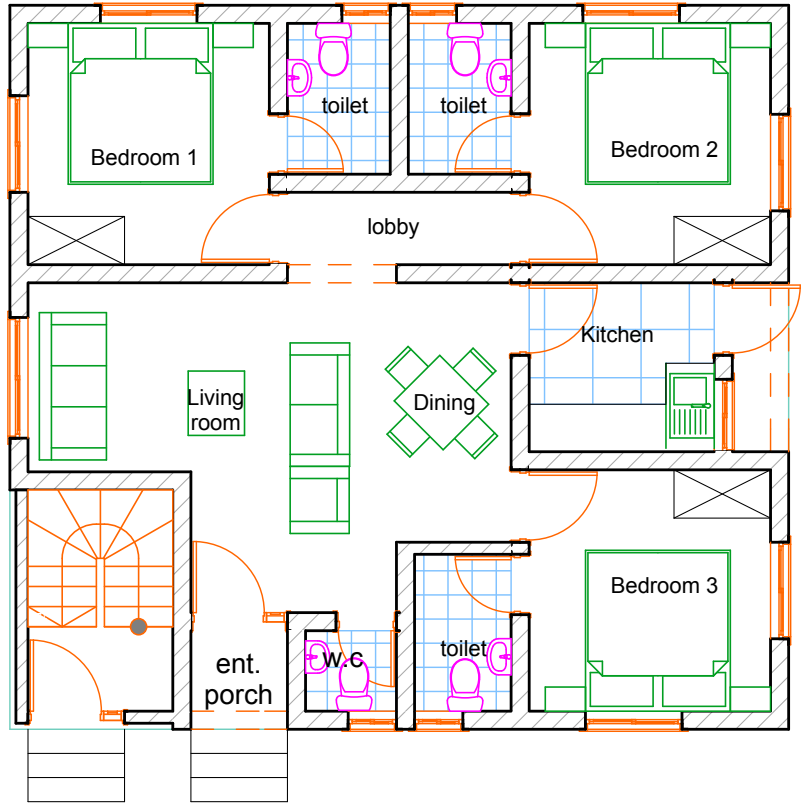
GROUND FLOOR (BLOCK 2)
